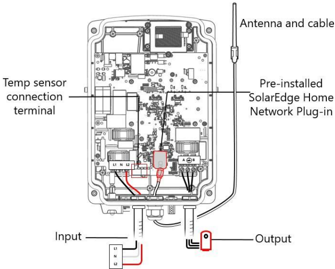
Figure 9: SolarEdge Home Hot Water Controller wire connections
