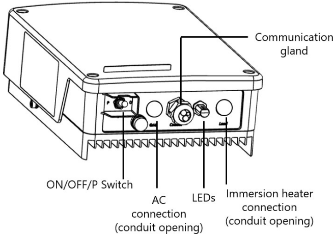
Figure 3: Device interfaces
