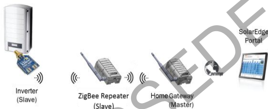
Figure 2: The SolarEdge ZigBee Repeater between the Home Gateway and Inverter
