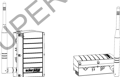
Figure 5: Antenna Orientation
