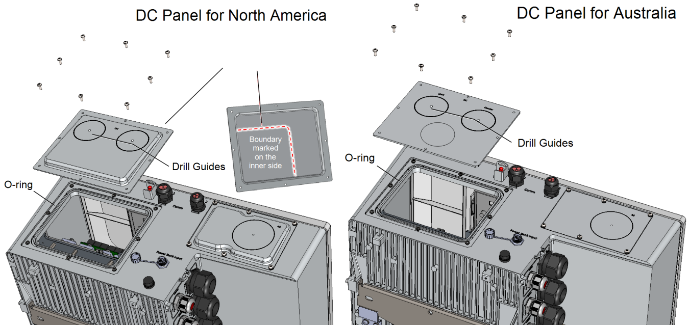
Figure 1: Removing the DC panel from the bottom of the Manager Unit
