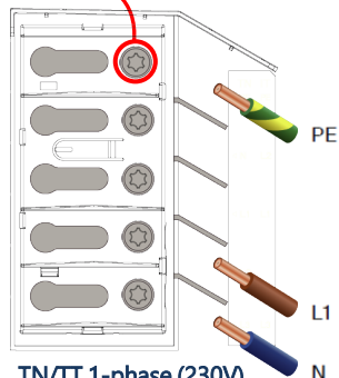
TN/TT 1-phase (230V)
