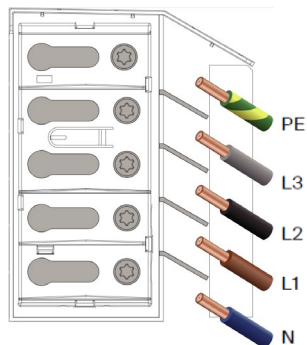
TN/TT 3-phase (3X 230V/400V)
