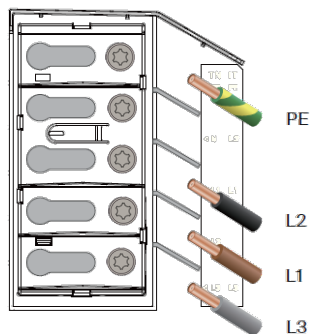
IT/TT 3-phase (3 x 230V)
