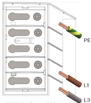
IT/TT 1-phase (230V)
