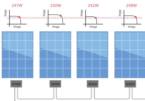
Figure 1: The partial shaded module is bypassed
