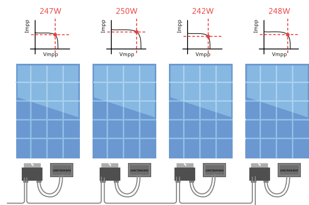
Figure 2: The partially shaded module contributes its power
