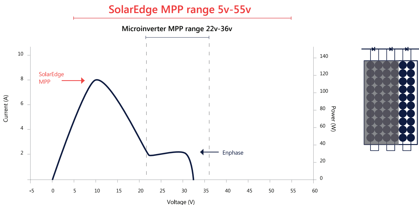
Figure 3: Microinverter module harvest is limited to the lower peak due to its narrow MPPT window
